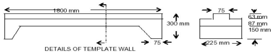
DETAILS OF TEMPLATE WALL
