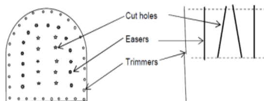
TYPICAL DRILLING PATTERN FOR ADIT / TUNNEL
