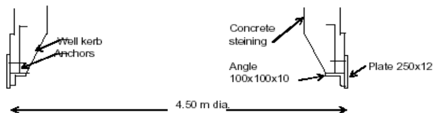
DETAILS OF FOUNDATION WELL CUTTING EDGE
