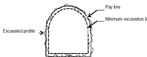
TYPICAL CROSS SECTION OF ADIT / TUNNEL
